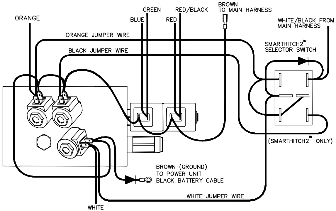
RT3 Straight Blade with SmartHitch2™ Manifold
