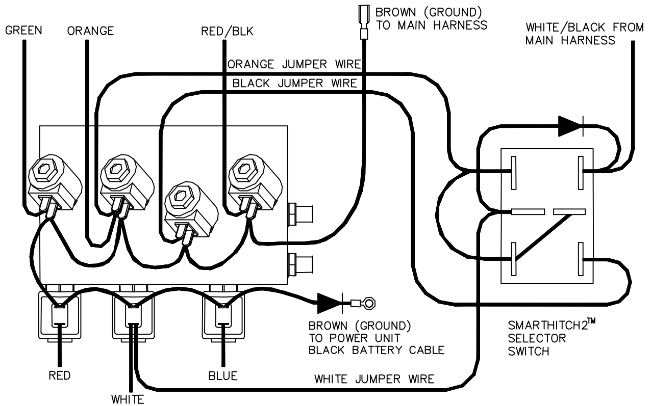
RT3 Power-V Blade with SmartHitch2™ Manifold
