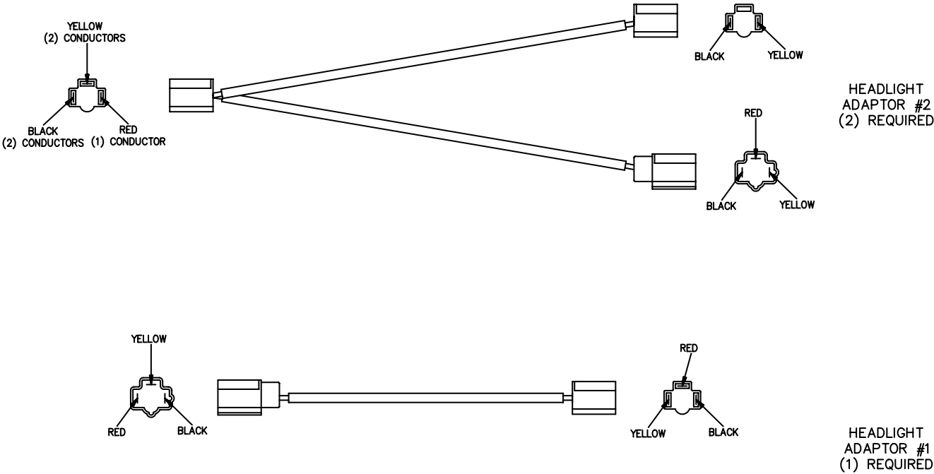
Figure 1. Headlight Adapter Kit, 1987 & Older Chevy/GMC
