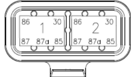
RELAY ORIENTATION IN HOLDER VIEW FROM TOP
