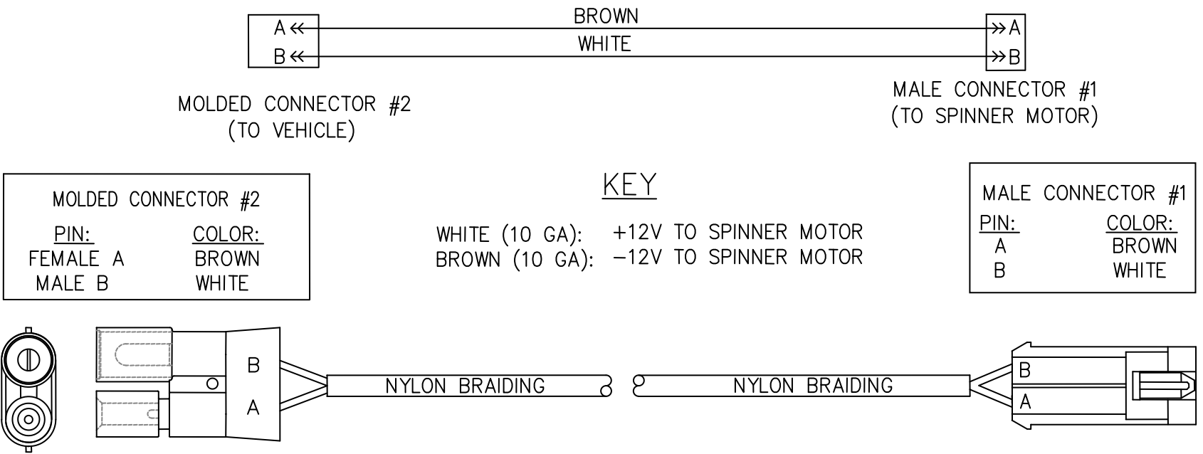
Figure 2. Spreader Side Harness Diagram (TGS06084)
