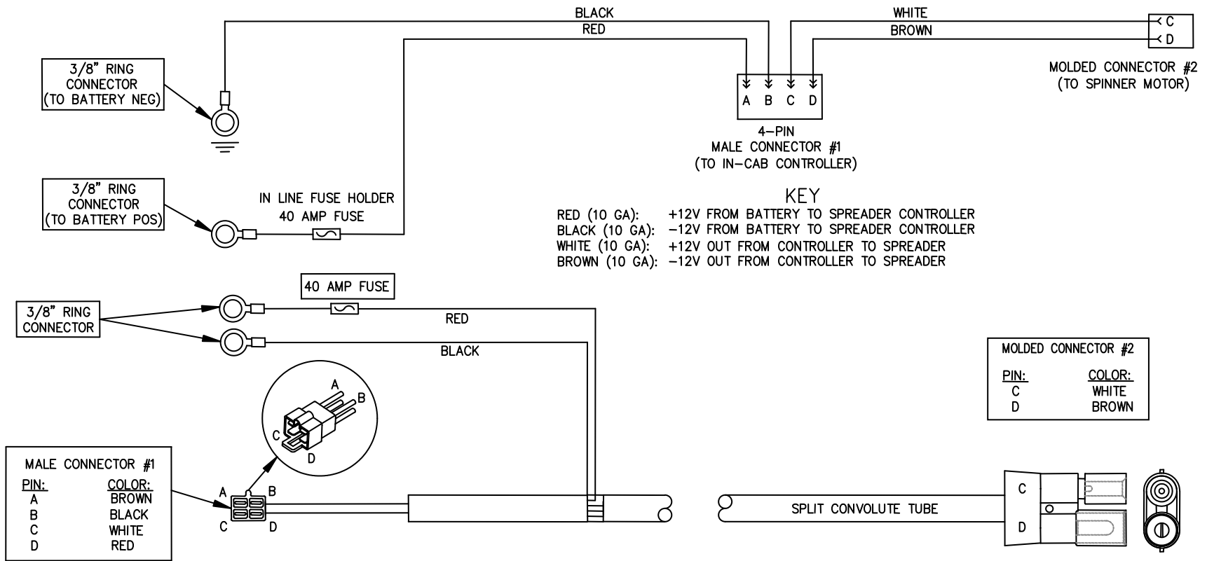
Figure 1. Vehicle Side Harness Diagram (TGS06085)
