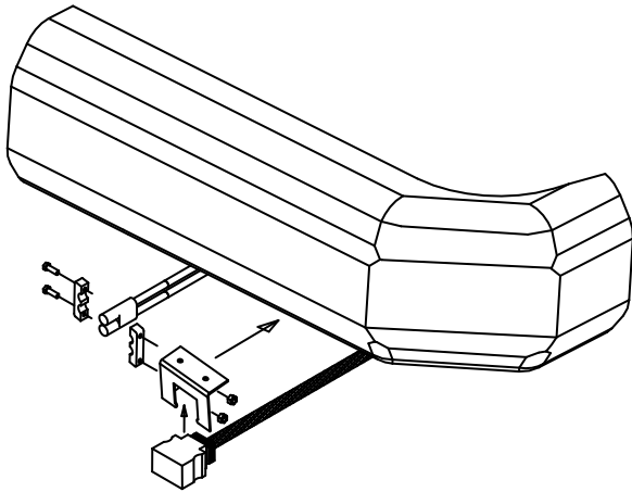
Figure 23. Vehicle Connections
