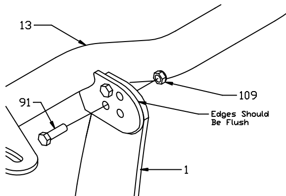
Figure 9. Light Bar Assembly. (Standard)
