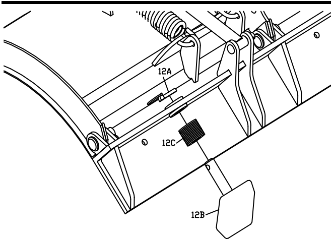
Figure 2. Install Shoe Assembly G10084
