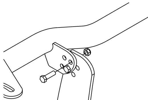
Figure 10. Light Bar Assembly Adjustment.
