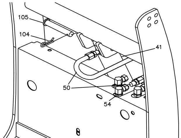
Figure 15. Installing SmartHitch2™ Hose G10120
