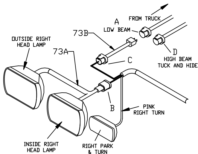
Figure 27. Dual Headlight Adapter Connections G10151
