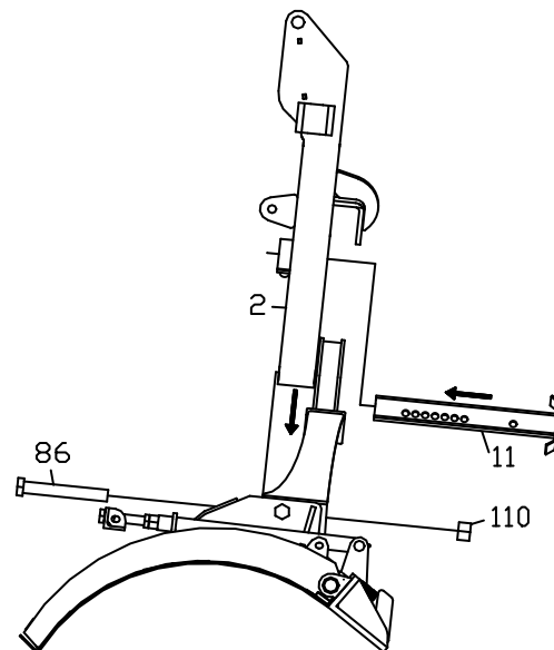
Figure 4. Install Pushframe and Kickstand. G10086
