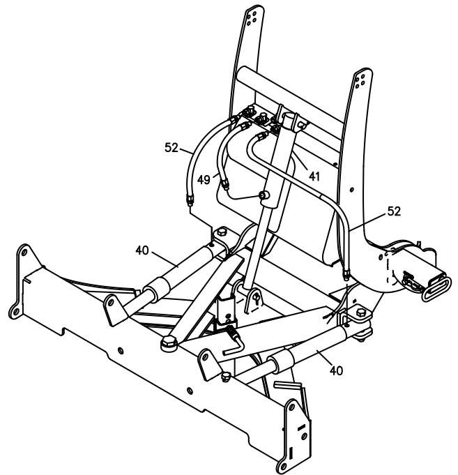
Figure 7. Hydraulic Connections
