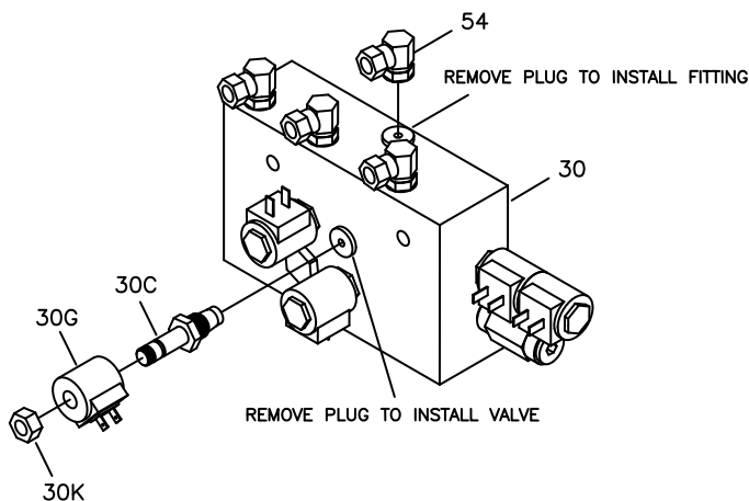
Figure 14. SmartHitch2™ Valve Installation G10130
