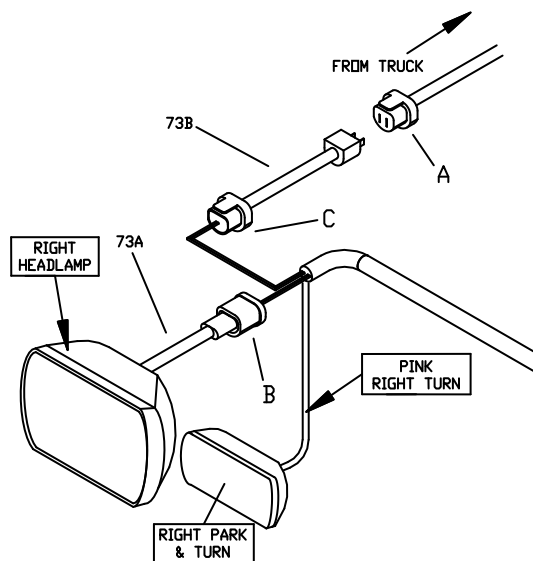
Figure 26. Single Headlight Adapter Connections G10149
