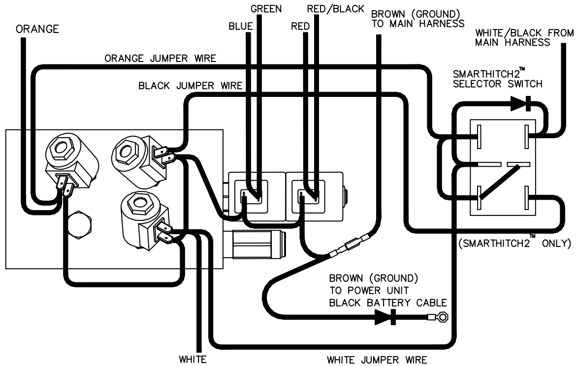
Figure 16. SmartHitch2™ Wiring Diagram
