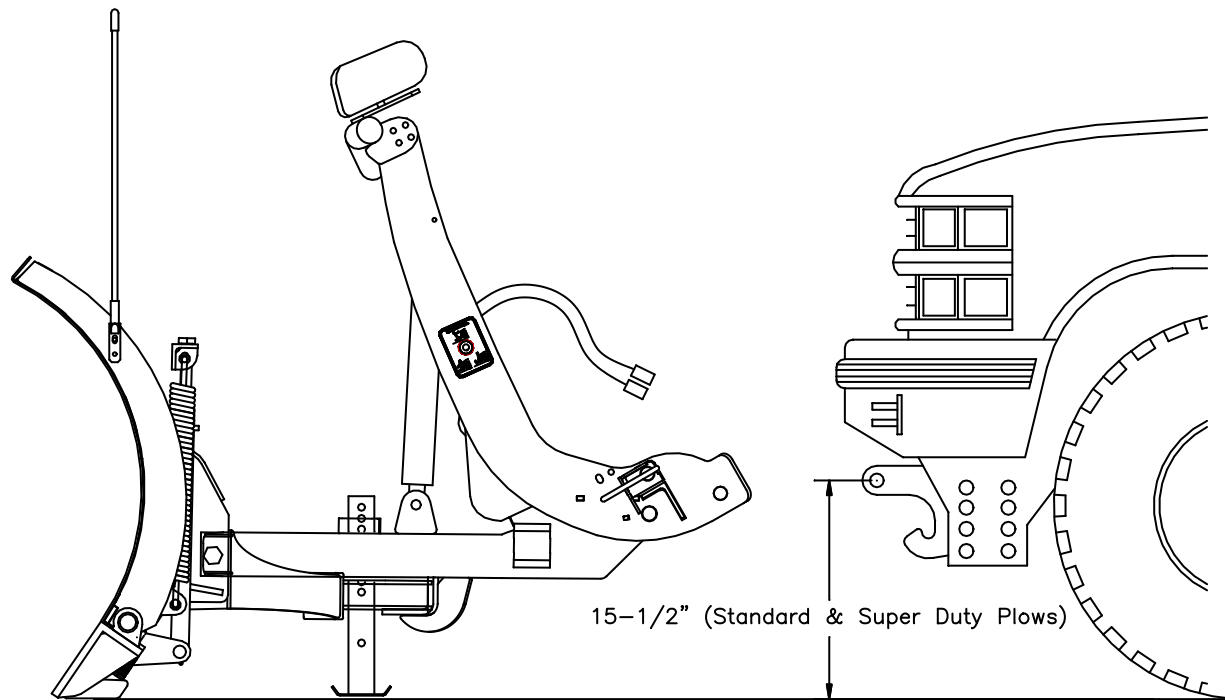
Figure 41. Recommended Pushbeam Height
