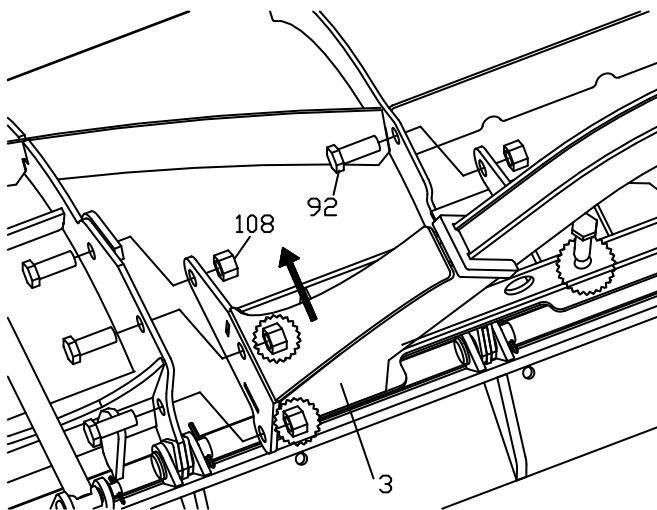
Figure 3. Install Pushframe Attachment Bar G10085
