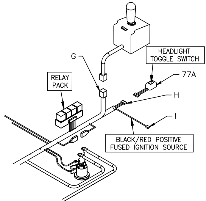
Figure 20. Internal Cab Wires G10144
