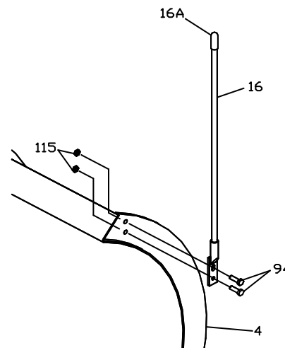
Figure 13. Assembly of Blade Guides. G10071
