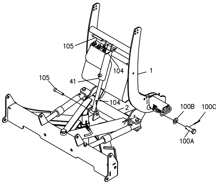
Figure 6. Lift Cylinder Installation
