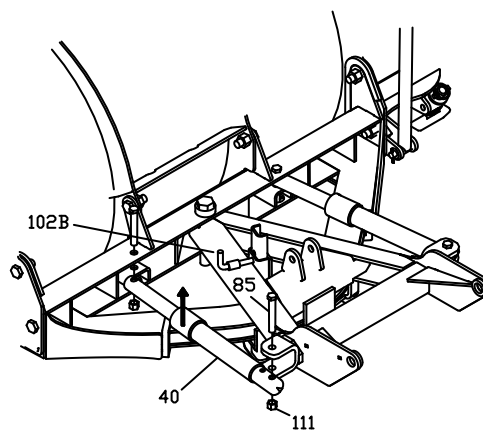
Figure 5. Install Angle Cylinders G10087
