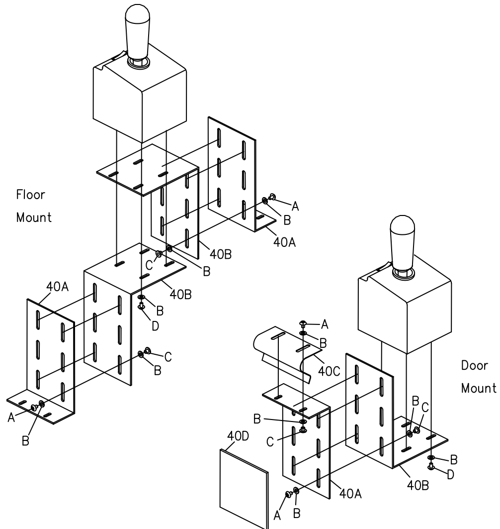
Figure 38. Joystick Control Universal Mounting Kit Components
