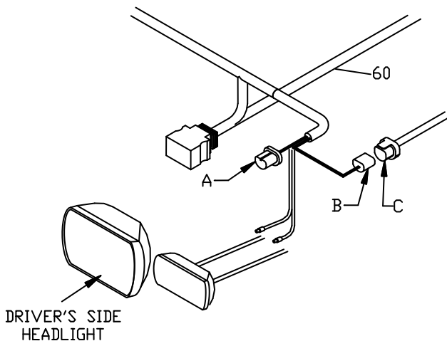
Figure 17. Driver Side Headlight G10140
