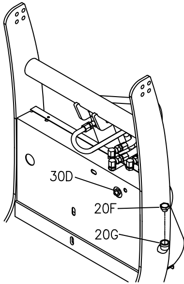
Figure 33. External Fill – Backside View G10124
