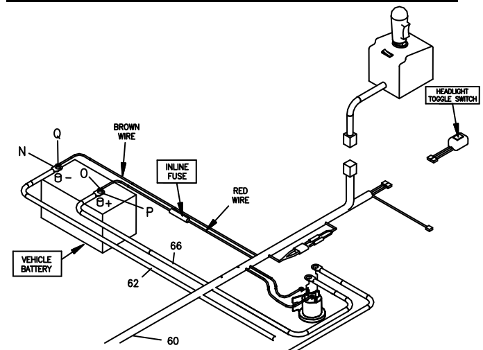
Figure 22. Battery Connections
