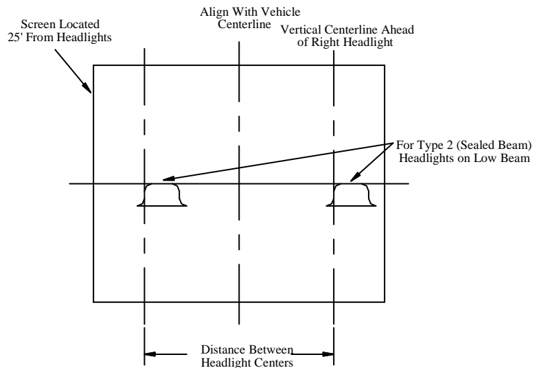
Figure 35. Headlight Aiming Procedure
