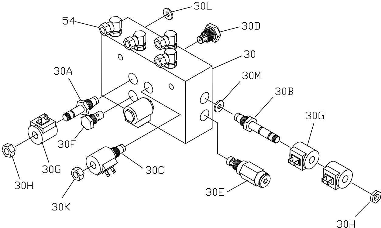
Figure 36. Straight Blade Manifold with SmartHitch2™ Parts Diagram G10072
