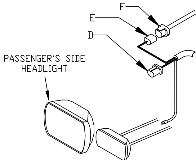
Figure 18. Passenger Side Headlight G10141
