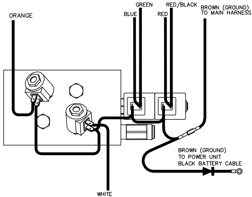
Figure 31. HYD07090 Standard Duty Manifold Wiring Diagram
