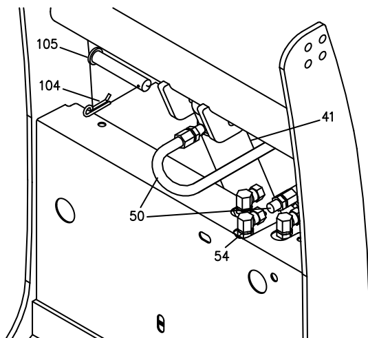
Figure 8. Connecting Hose
